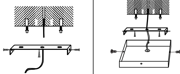
Ceiling installation diagram
